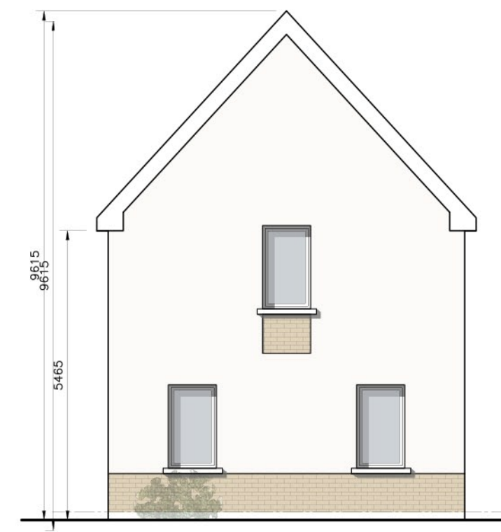
Gable Elevation
