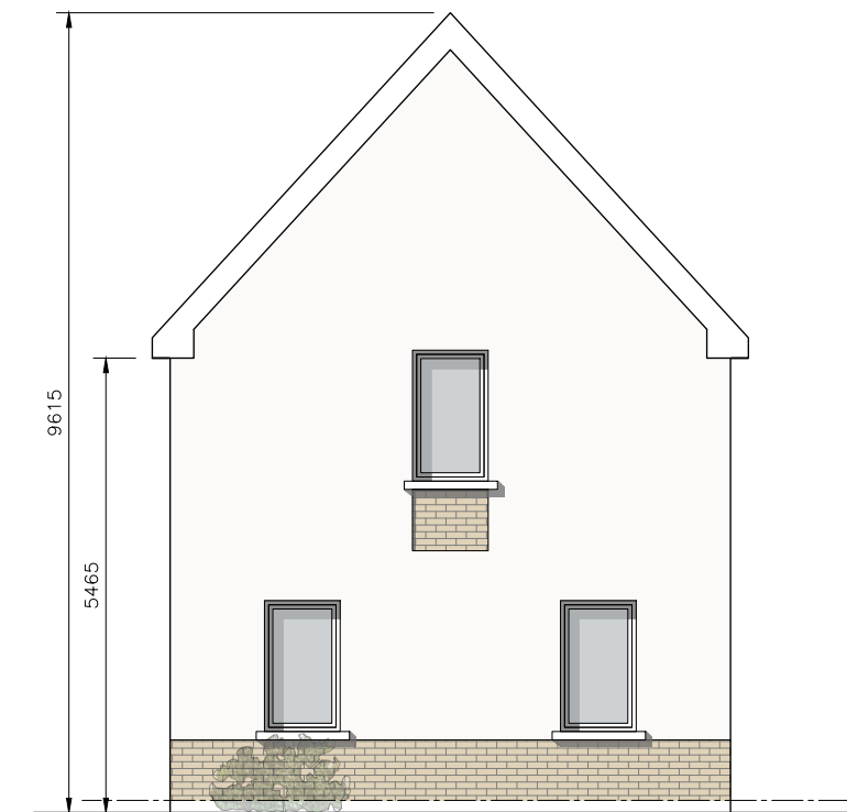
Gable Elevation
