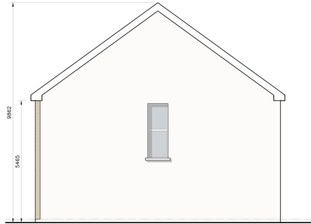
Gable Elevation
